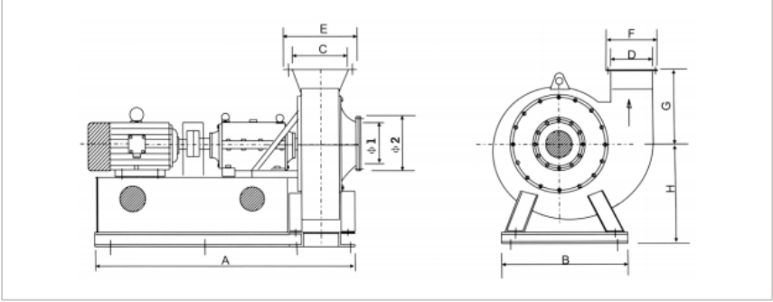
9-19型D式风机外形及安装尺寸 D type Fan external from and mounted dimension
