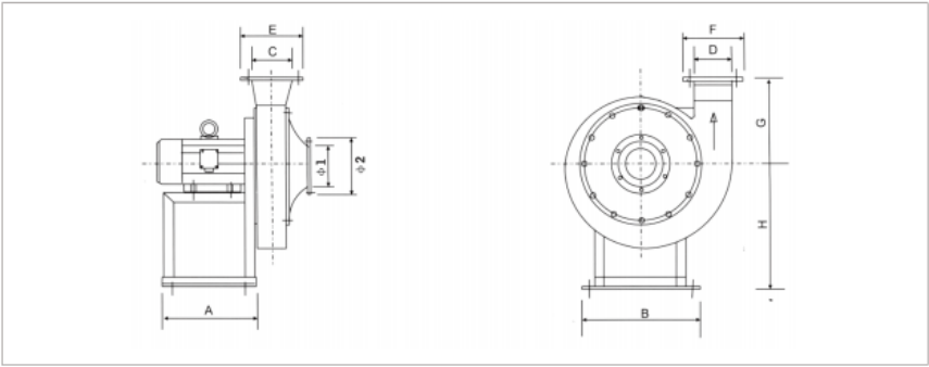
9-19型A式风机外形及安装尺寸 A type Fan external from and mounted dimension
