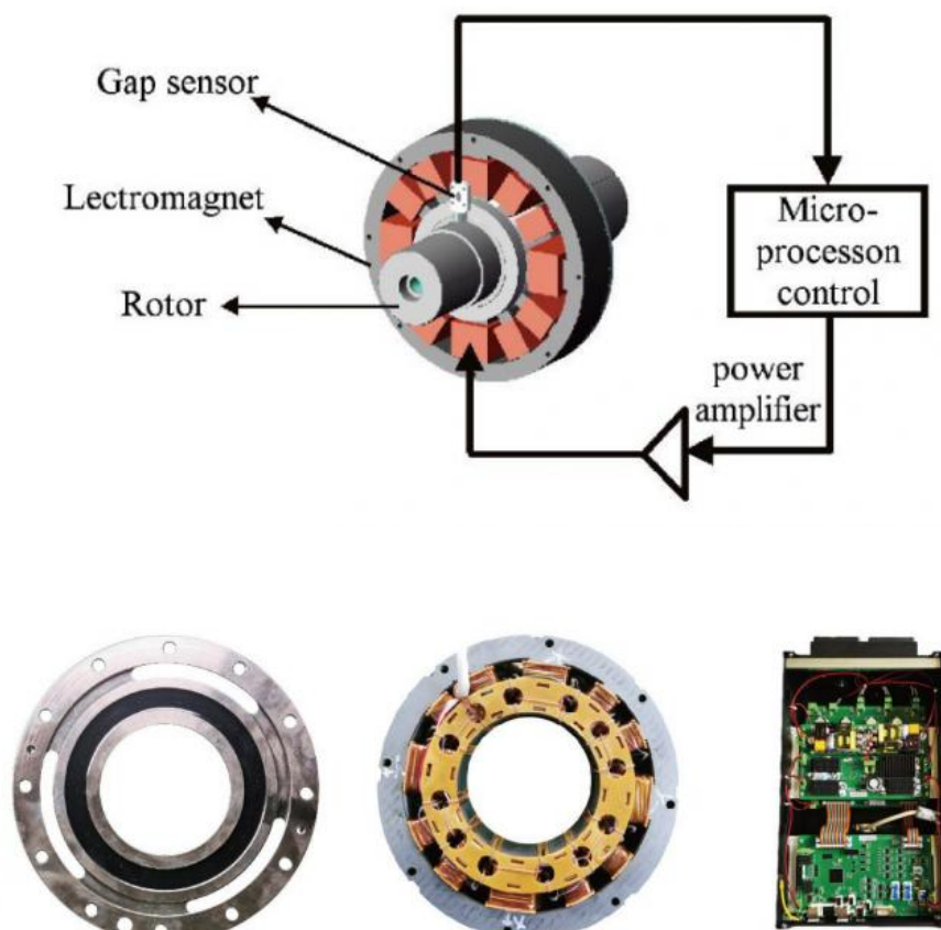
magnetic levitation bearing
